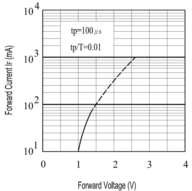
Fig.4 Forward Current
